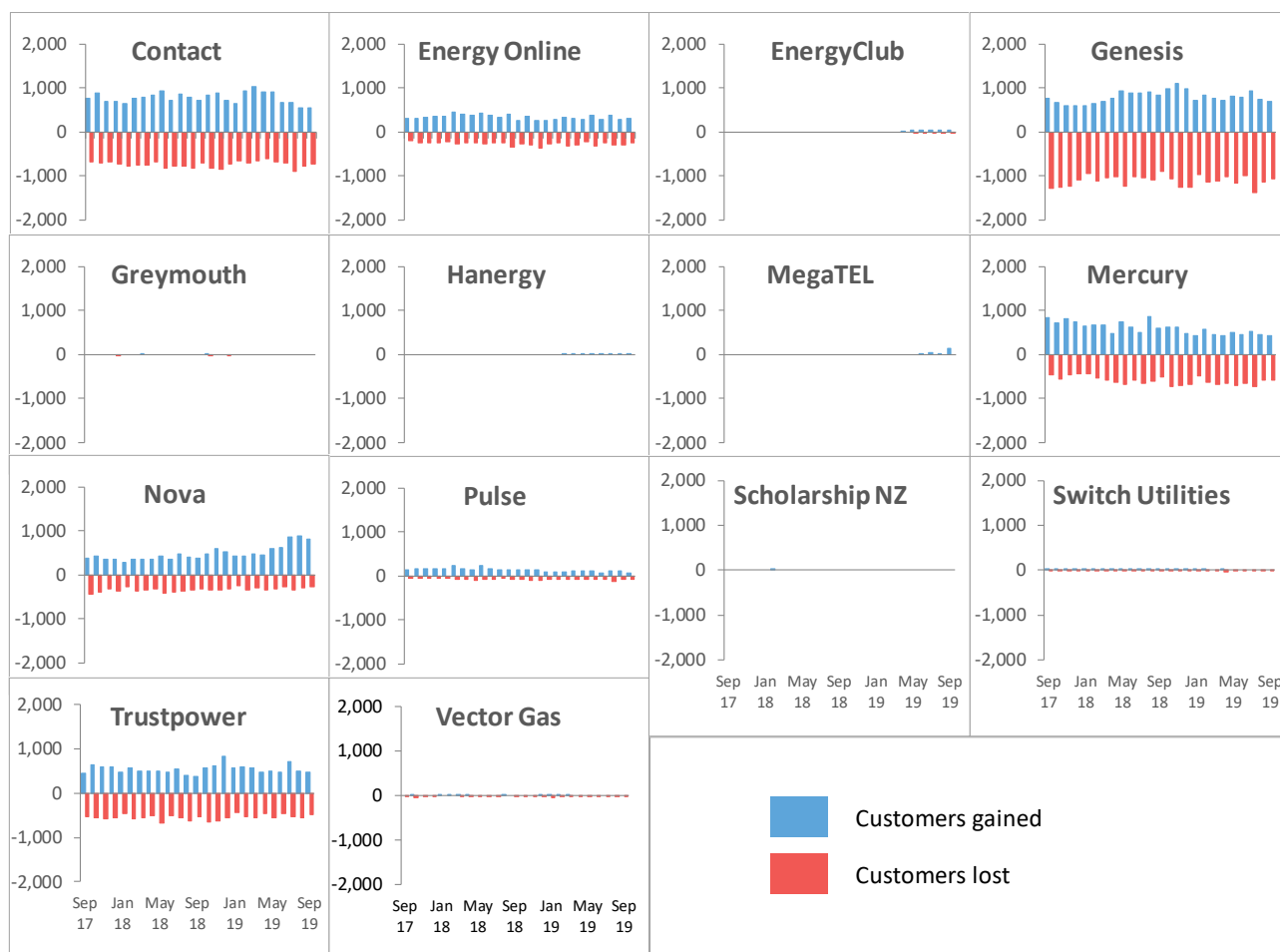
Chart 16: Switching activity by retailer
