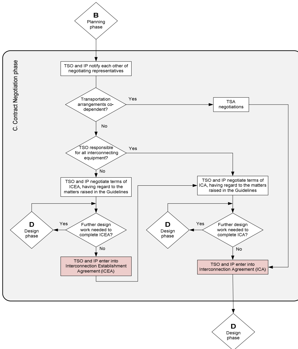
Figure 6 – Contract Negotiation Phase Process
