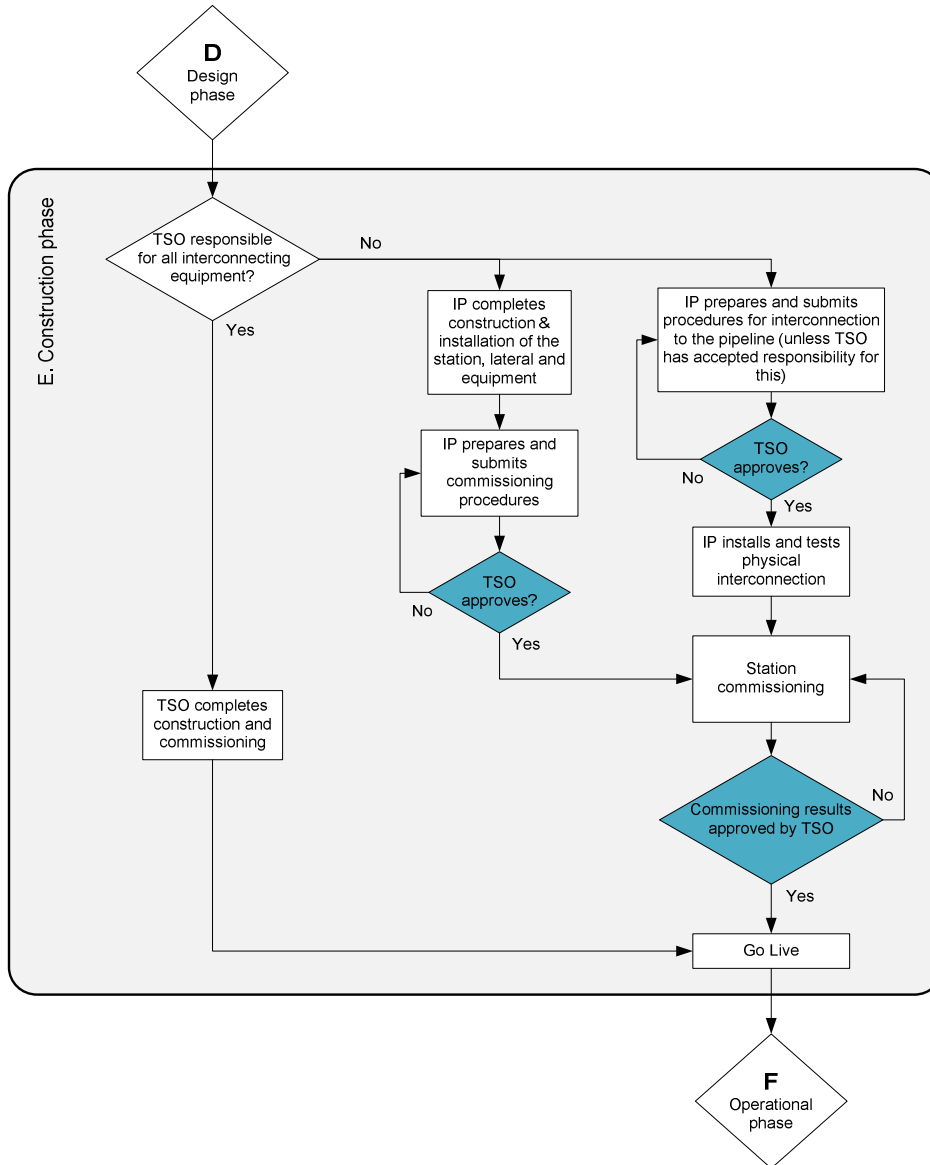
Figure 8 - Construction Phase Process
